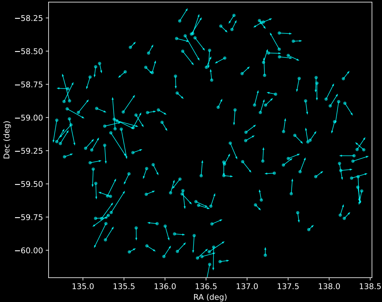
GALAH DR4 Noise Stream Proper Motion Vectors (n=154)
