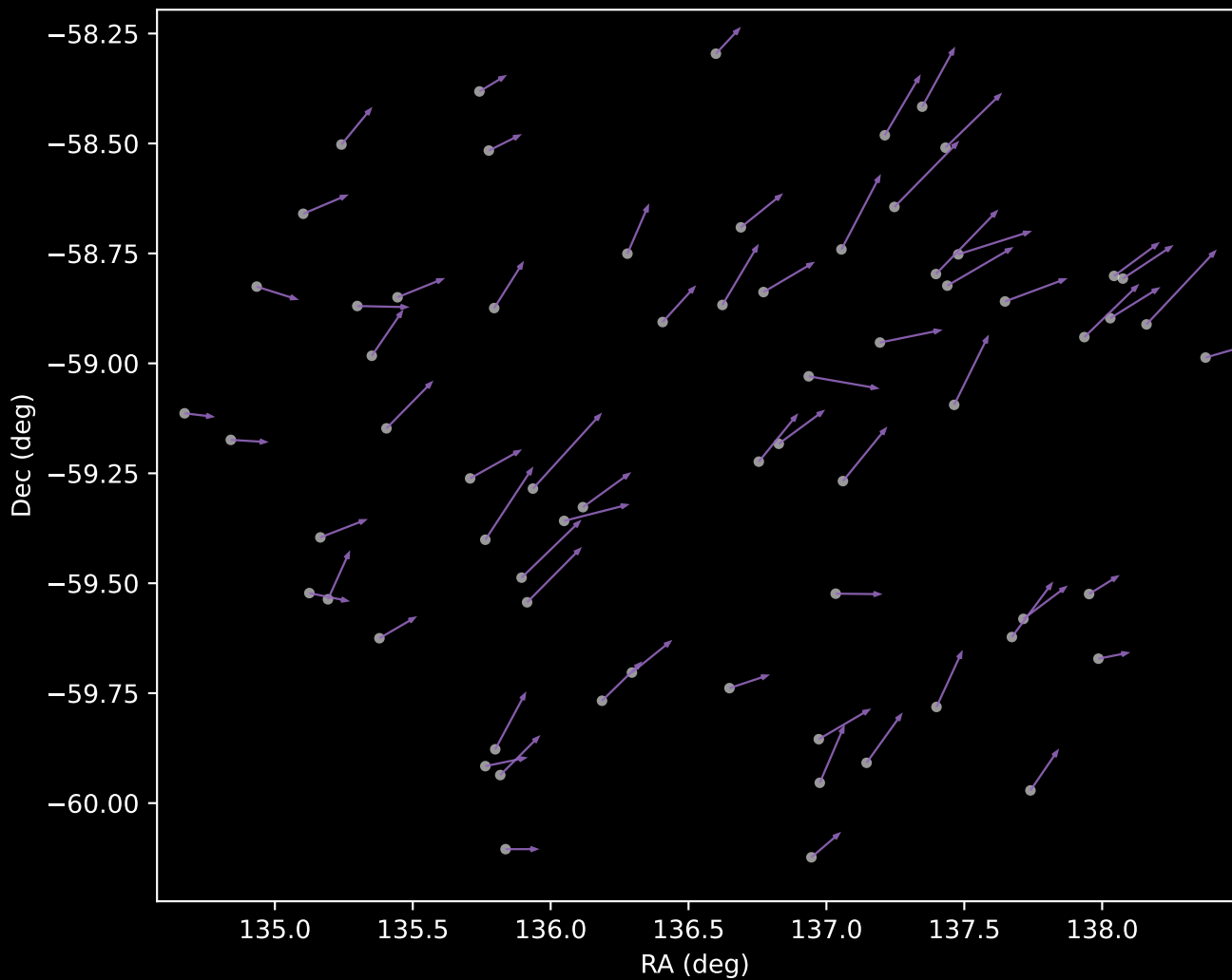
GALAH DR4 Cluster 8 Proper Motion Vectors (n=68)
