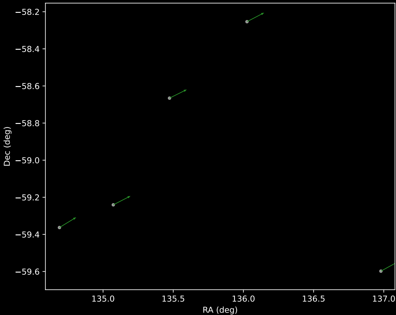
GALAH DR4 Cluster 4 Proper Motion Vectors (n=5)
