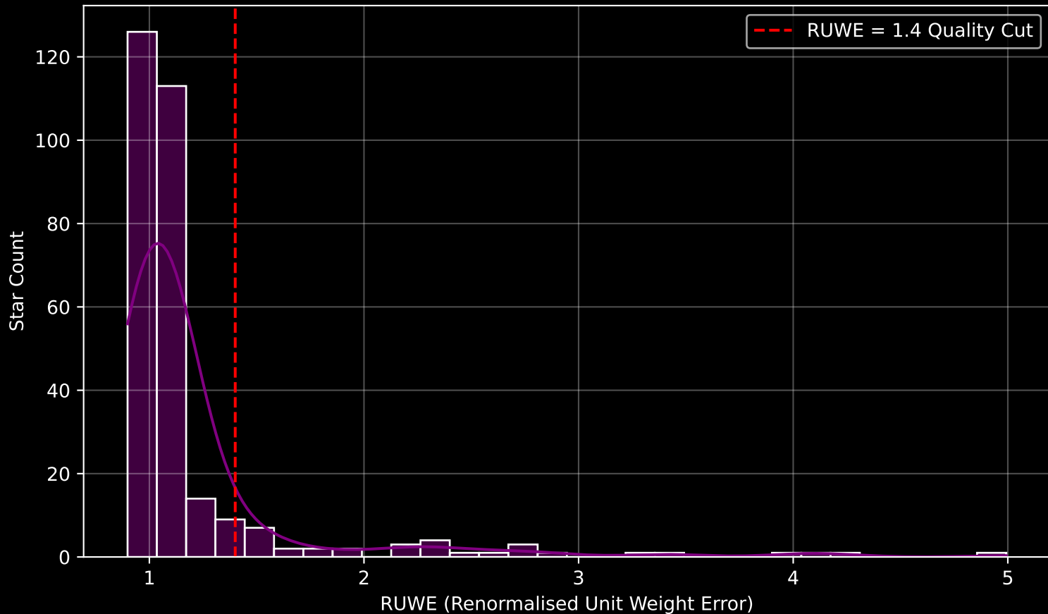
GALAH DR4 Field [6923] RUWE Distribution (n= 294)
