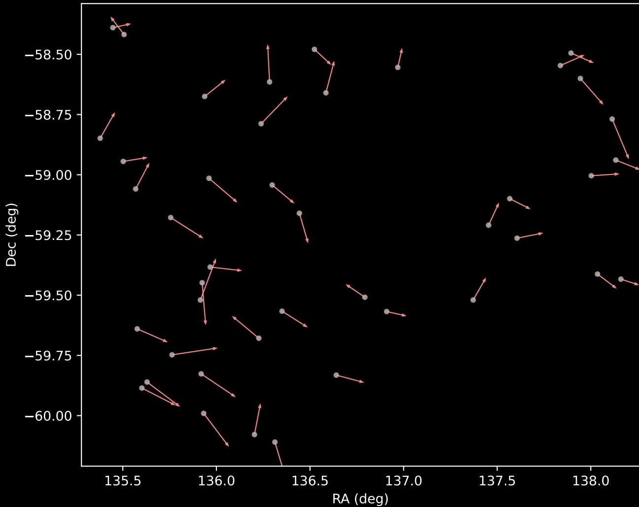
GALAH DR4 Cluster 7 Proper Motion Vectors (n=43)
