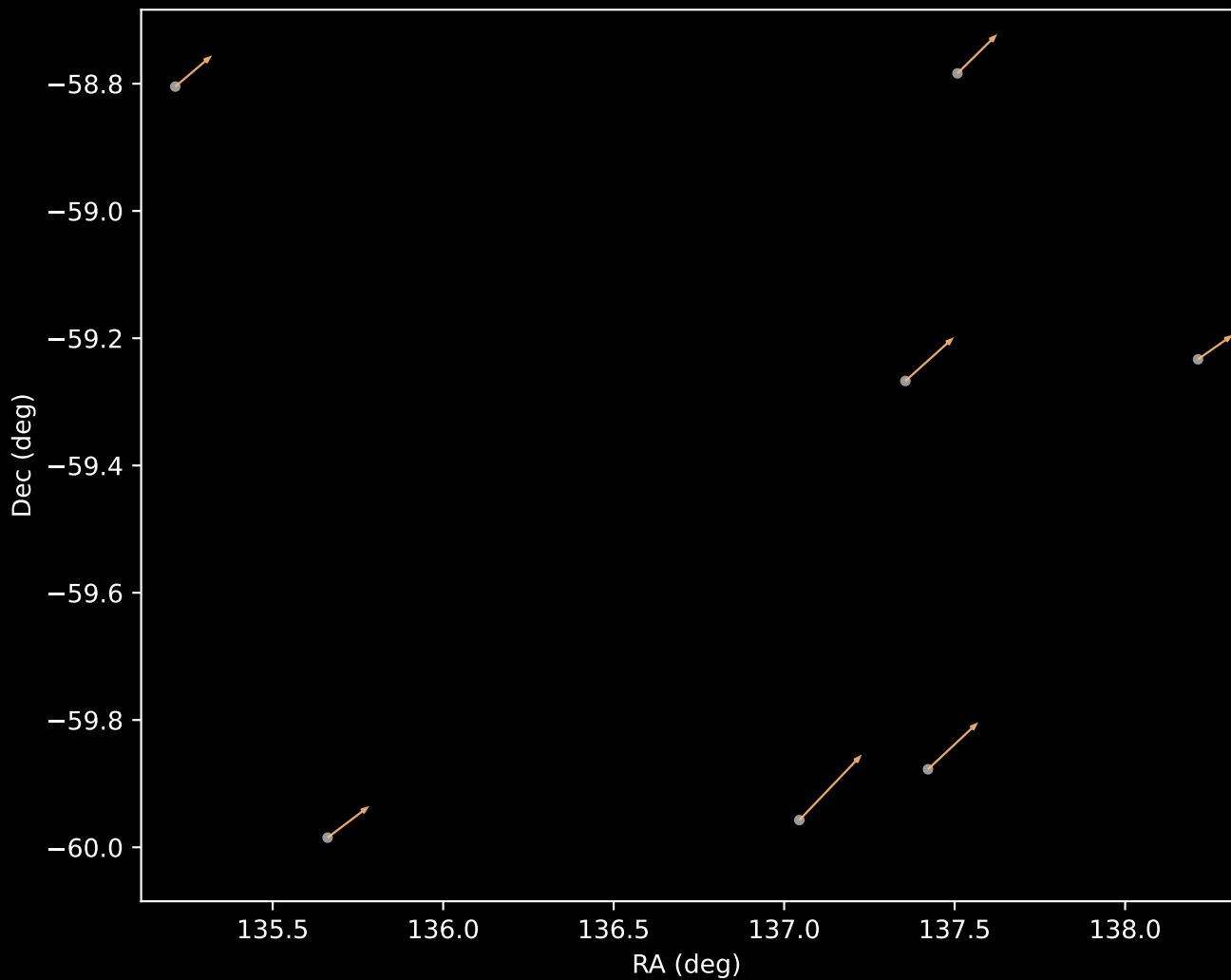
GALAH DR4 Cluster 3 Proper Motion Vectors (n=7)
